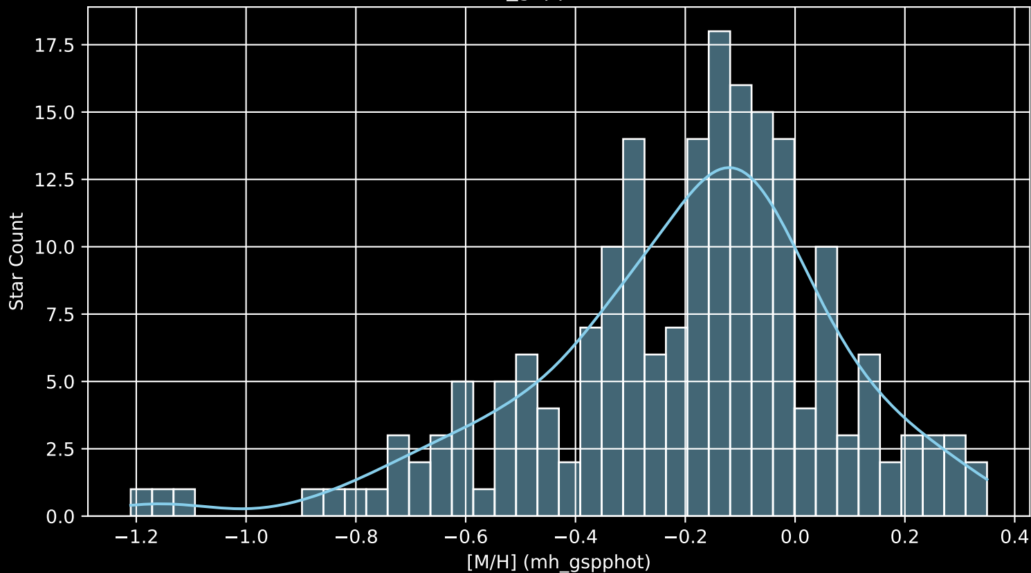
APOGEE DR17 Field: [075-35_MGA [M/H] (mh_gspphot) (n= 195)
