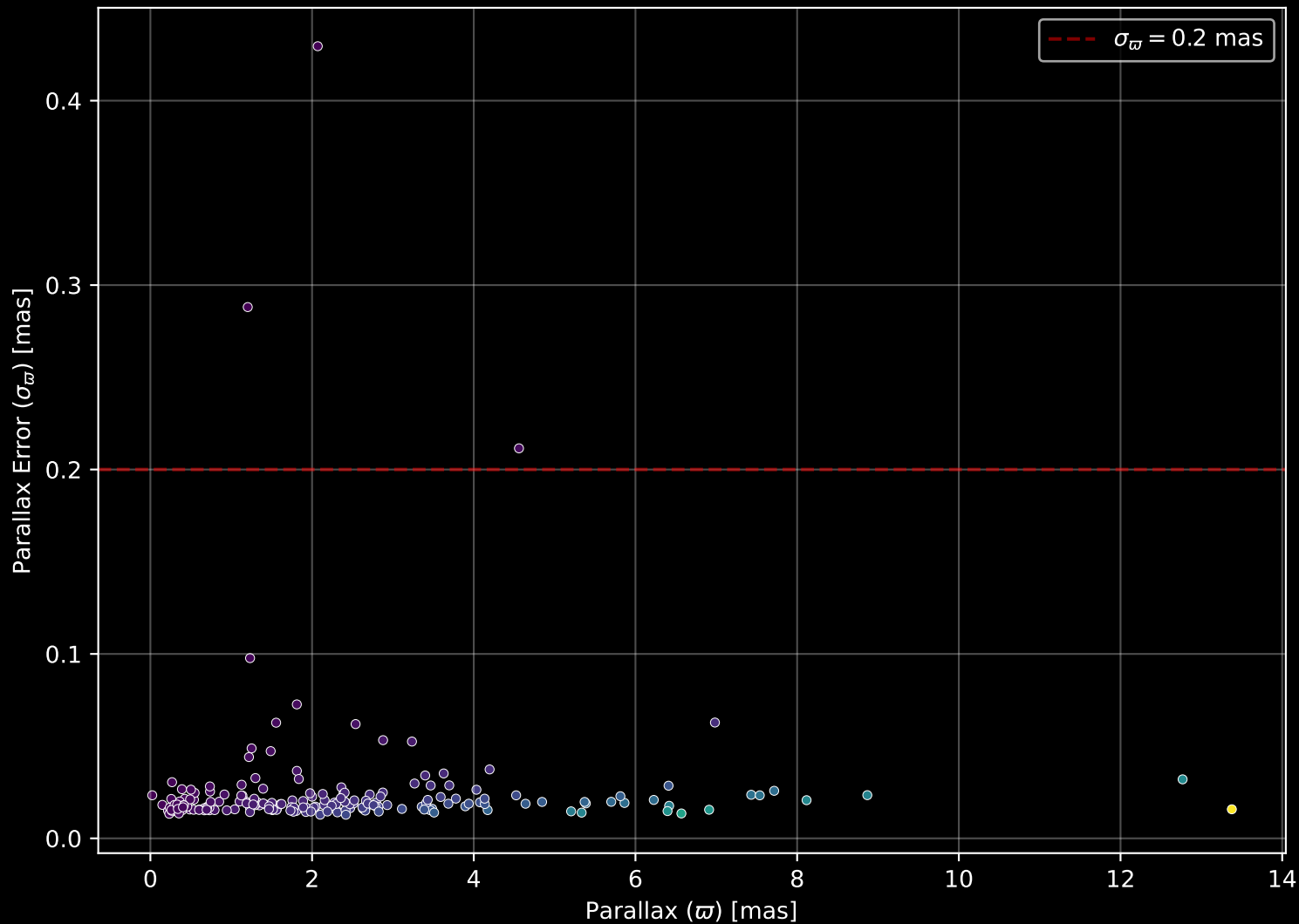
APOGEE DR17 Field: [075-35_MGA] Parallax Quality (n= 199)
