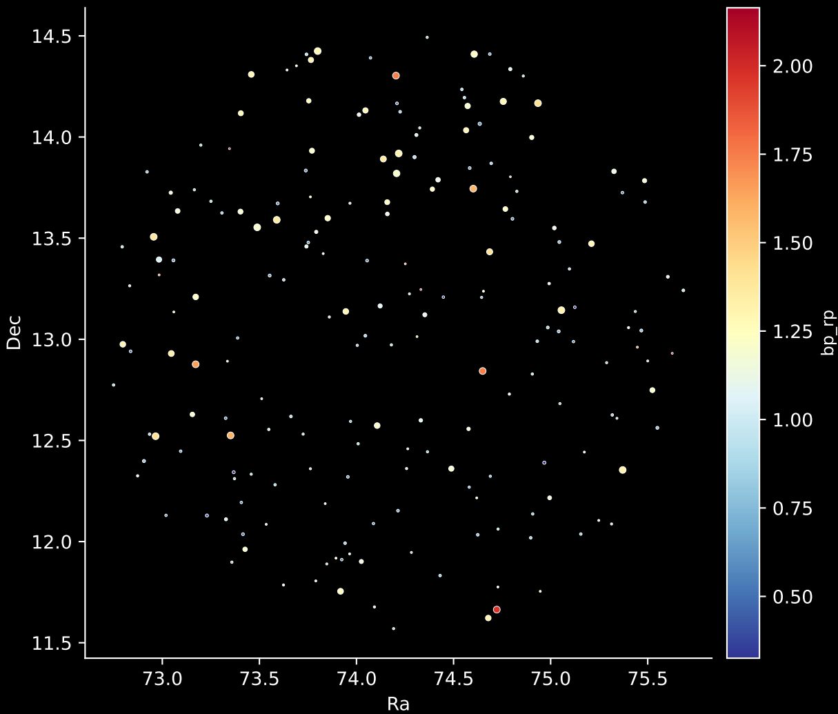
APOGEE DR17 Field: [075-35_MGA] Stars: 199
