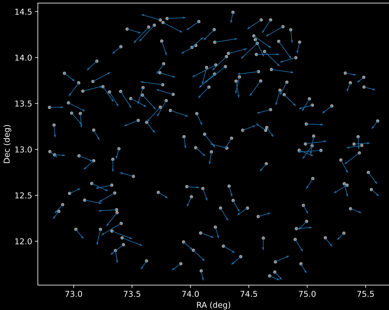
APOGEE DR17 Cluster 0 Proper Motion Vectors (n=156)
