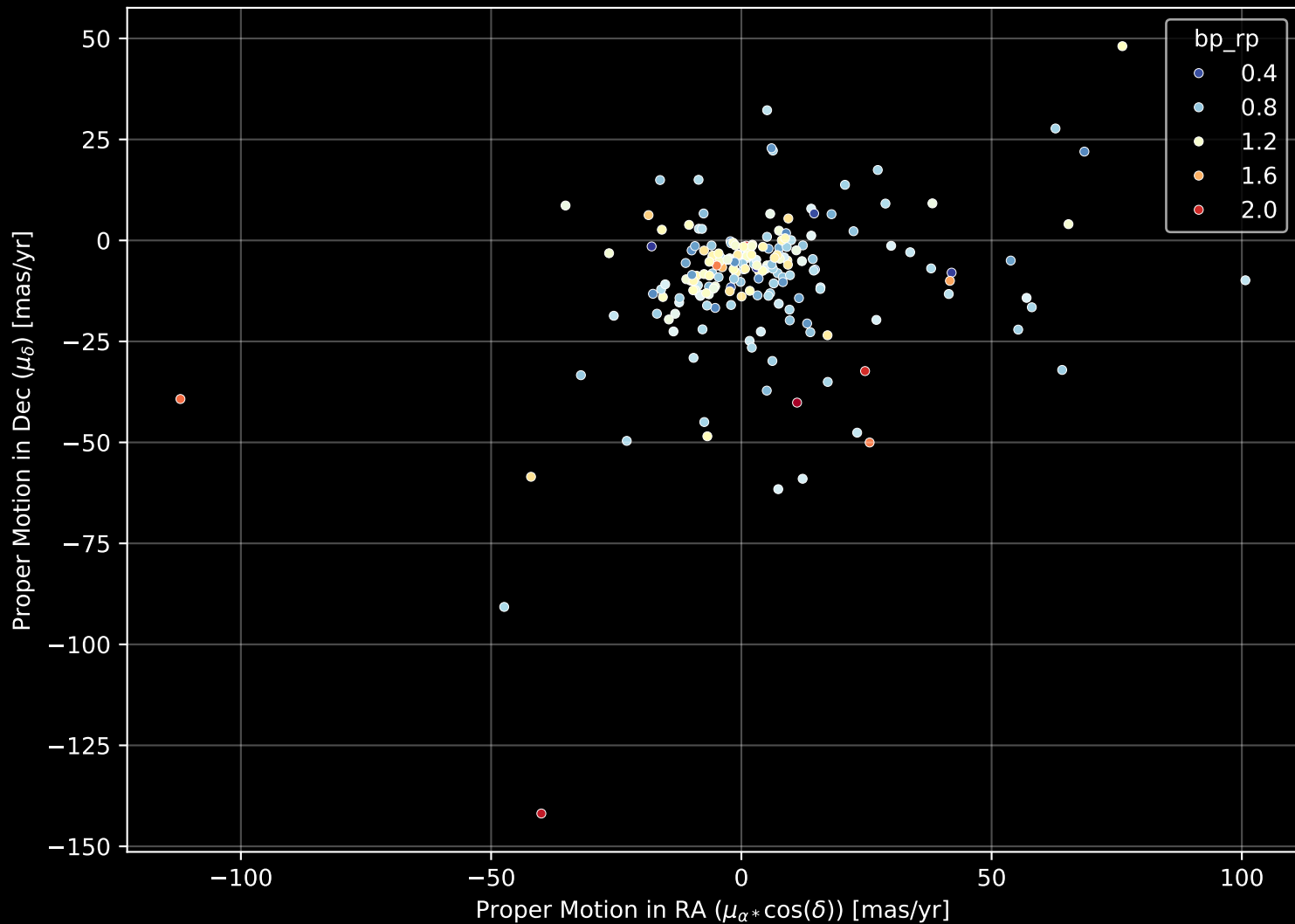
APOGEE DR17 Field: [075-35_MGA] Proper Motion Diagram (n= 199)
